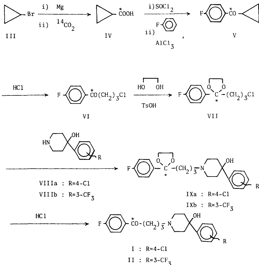
Fig. 1. Scheme for the syntheses of haloperidol-1- 14 C and trifluoperidol-1- 14 C
